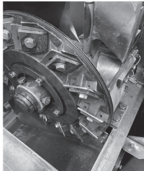
Figure 3: Rotating blade of a commercial katsuobushi shaving machine
